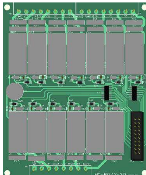
Relay PCB
